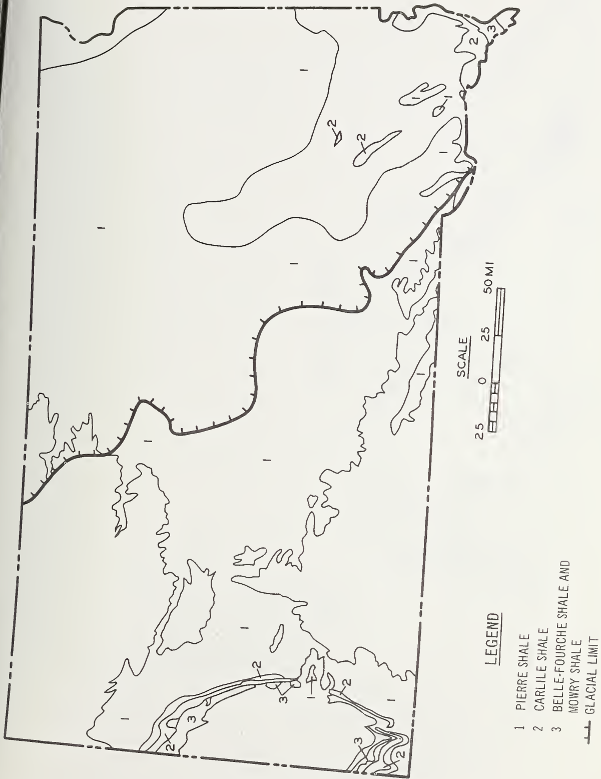
Figure 15. Occurrence of problem shales, South Dakota.
